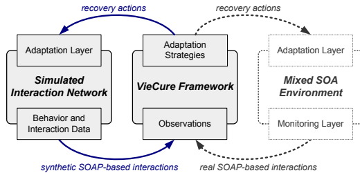
Figure 6. Simulation setup.
