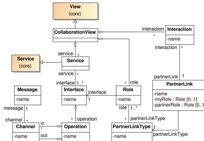
Figure 4. Collaboration view meta-model
