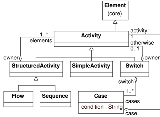
Figure 3. Orchestration view meta-model
