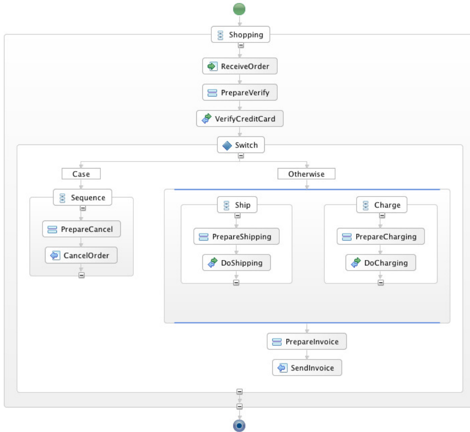
Figure 7. The shopping case study
