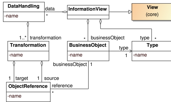
Figure 5. Information view meta-model
