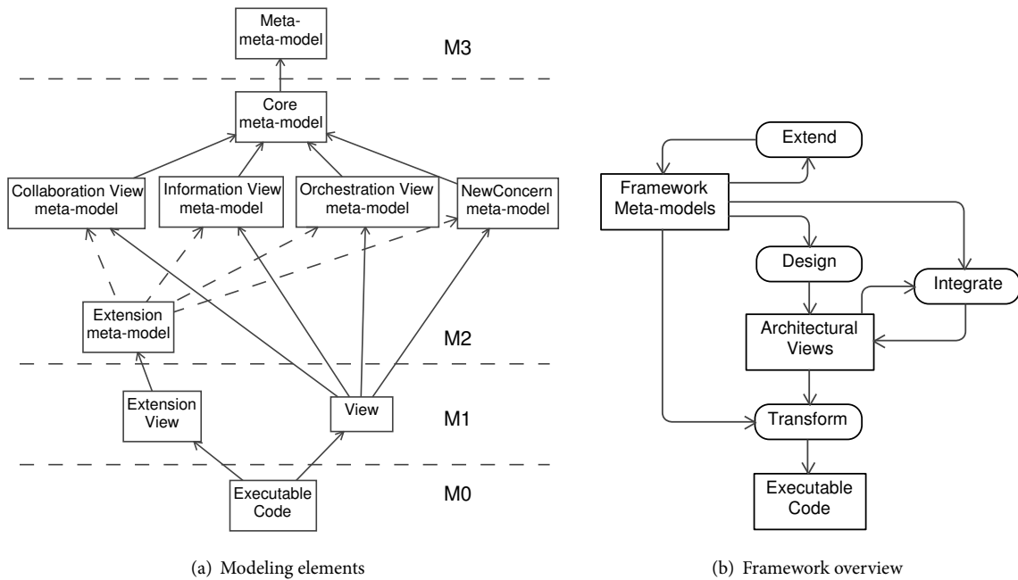
Figure 1. View-based model-driven framework
