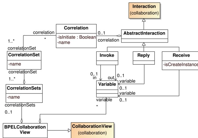
Figure 6. An extension of the collaboration view
