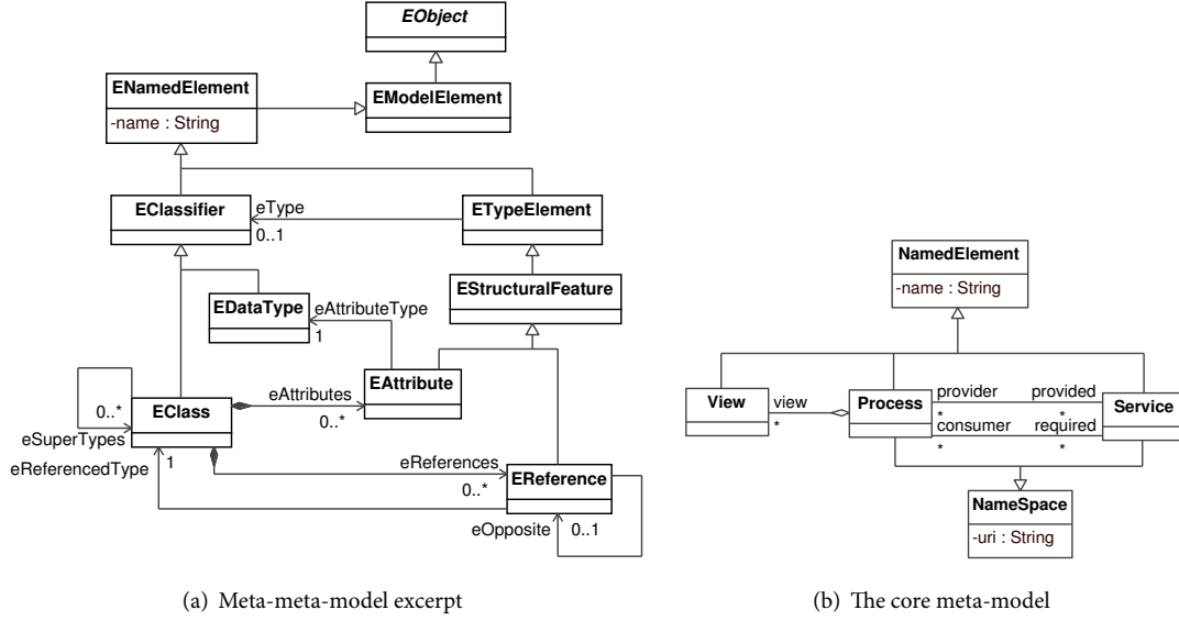
Figure 2. Meta-meta-model and the Core meta-model
