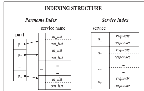
Figure 2. Index Structure.
