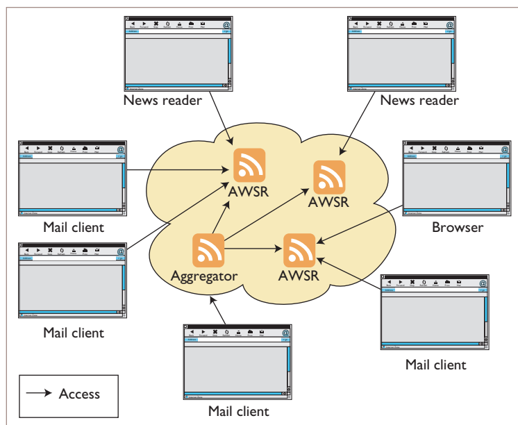
Figure 2. Client- and server-side AWSR aggregation. The aggregator unifies three AWSR feeds and then provides a single feed back to a single client; the other clients connect directly to AWSR registries.
