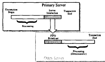
Figure 7. Primary copy, constant interaction, non-voting
