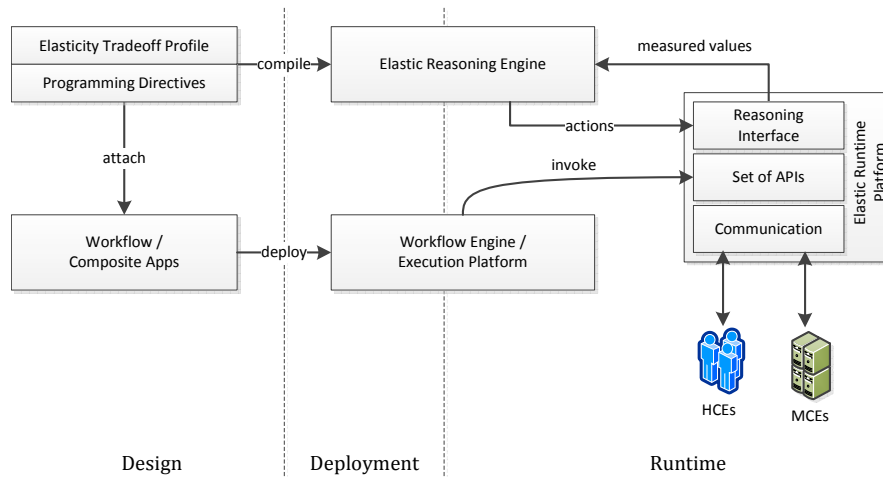
Fig. 1.4 Steps in programming and executing hybrid services in VieCOM
