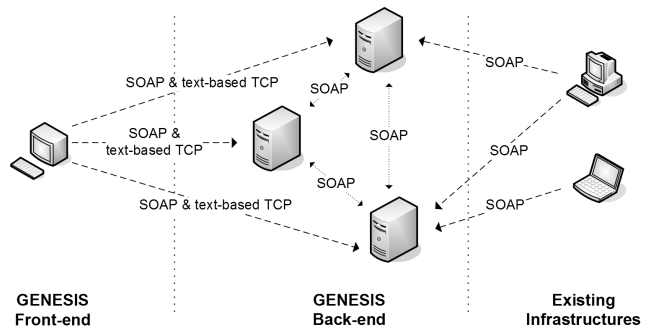
Figure 3. Communication in the testbed
