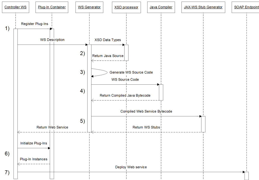
Figure 4. Web service generation
