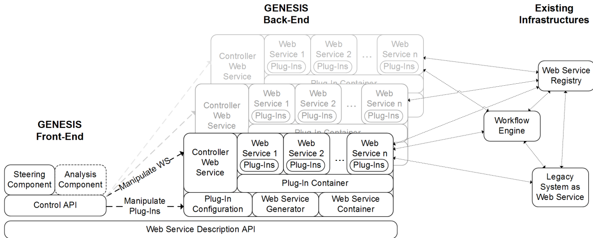
Figure 2. Architecture of GENESIS
