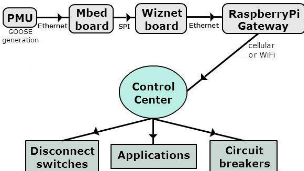
Figure 44: Gateway for the GOOSE
