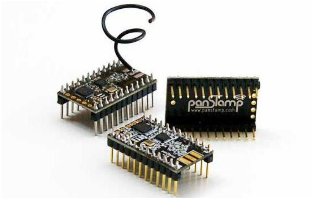
Figure 17: PanStamp modules [39]
