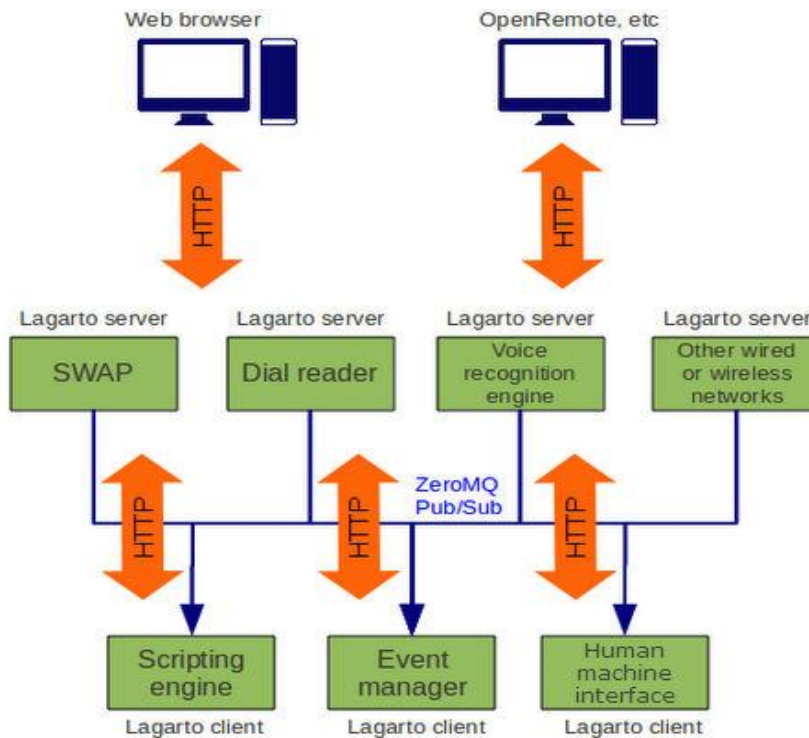
Figure 20: Lagarto architecture [41]
