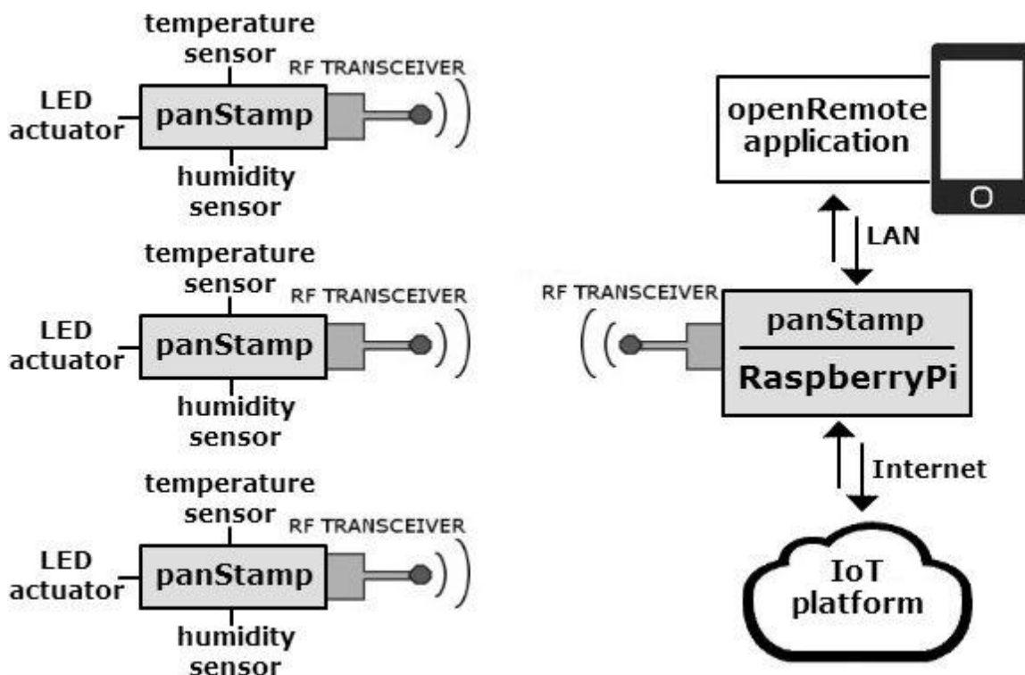
Figure 29: Implemented end-device network with Internet connectivity
