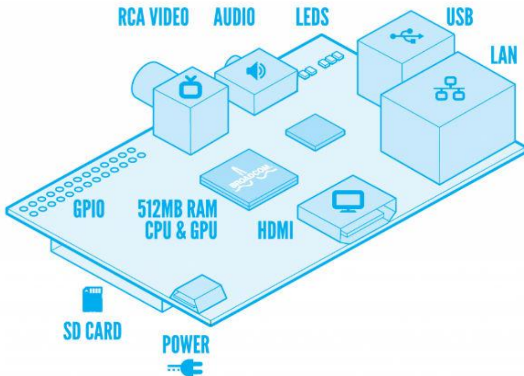
Figure 25: Raspberry Pi (model B) design [48]
