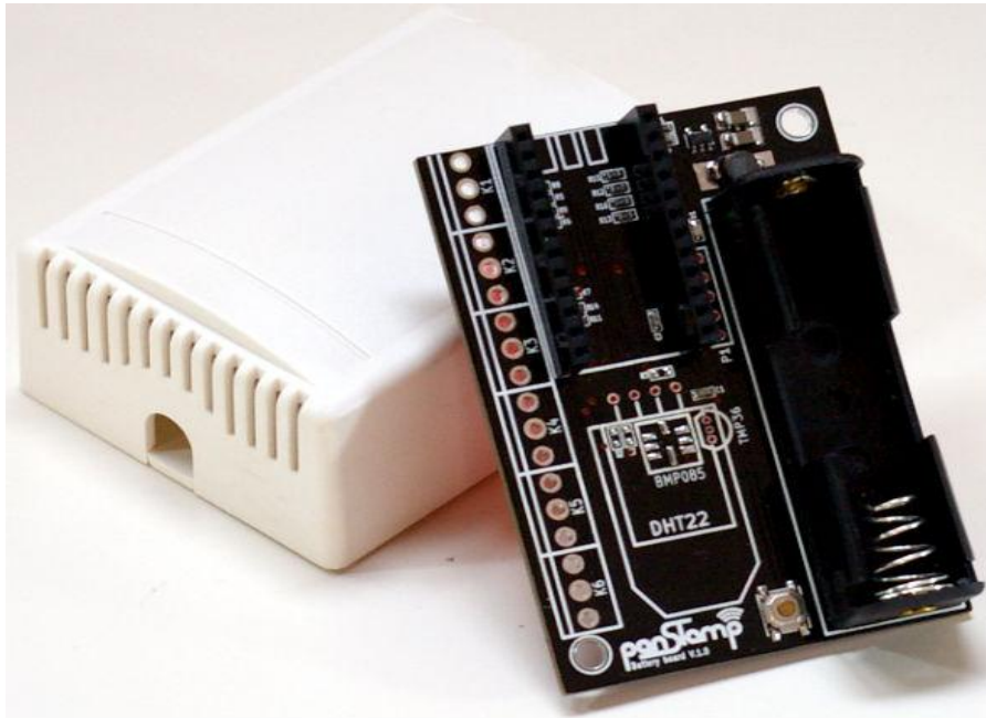
Figure 18: PanStamp base board [34]
