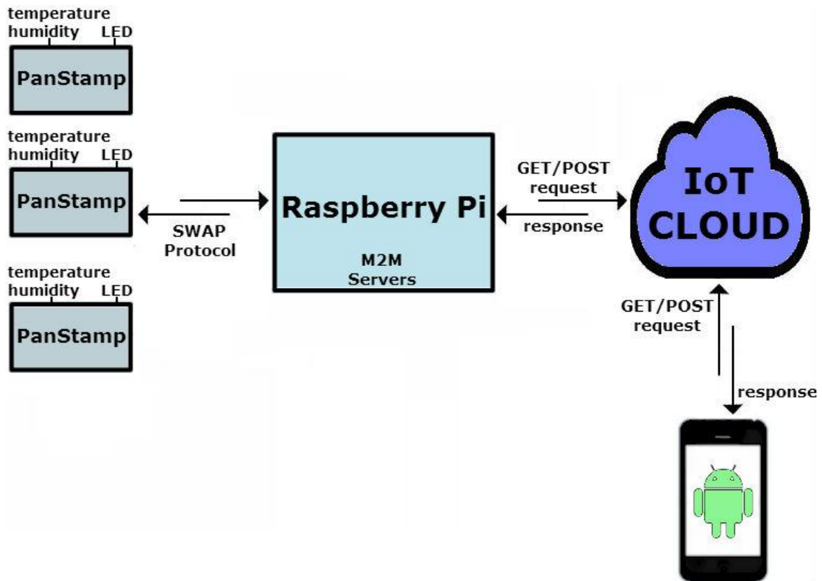
Figure 35: Android connectivity to the end-devices
