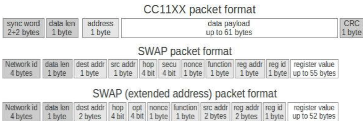
Figure 21: SWAP packet structure [44]
