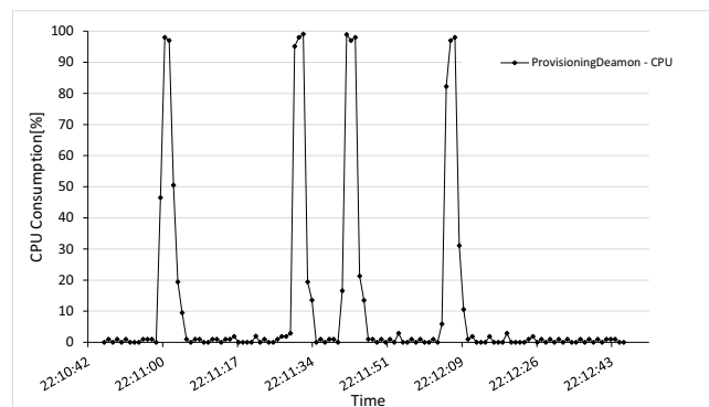
Fig. 10. CPU consumption of the ProvisioningDaemon.
