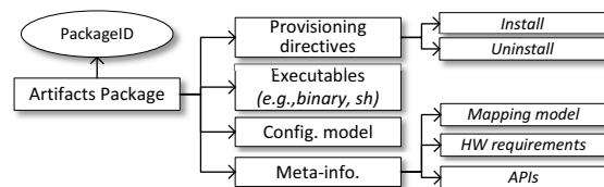
Fig. 4. Artifacts package structure.
