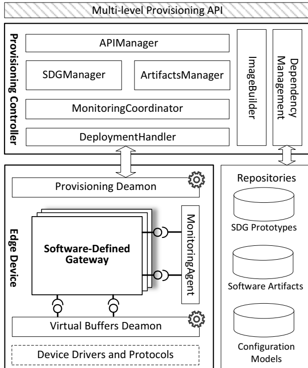
Fig. 2. Architecture overview of the provisioning middleware.
